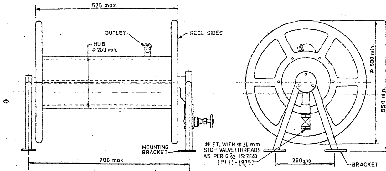
FIG. 2 HOSE REEL HORIZONTAL TYPE
