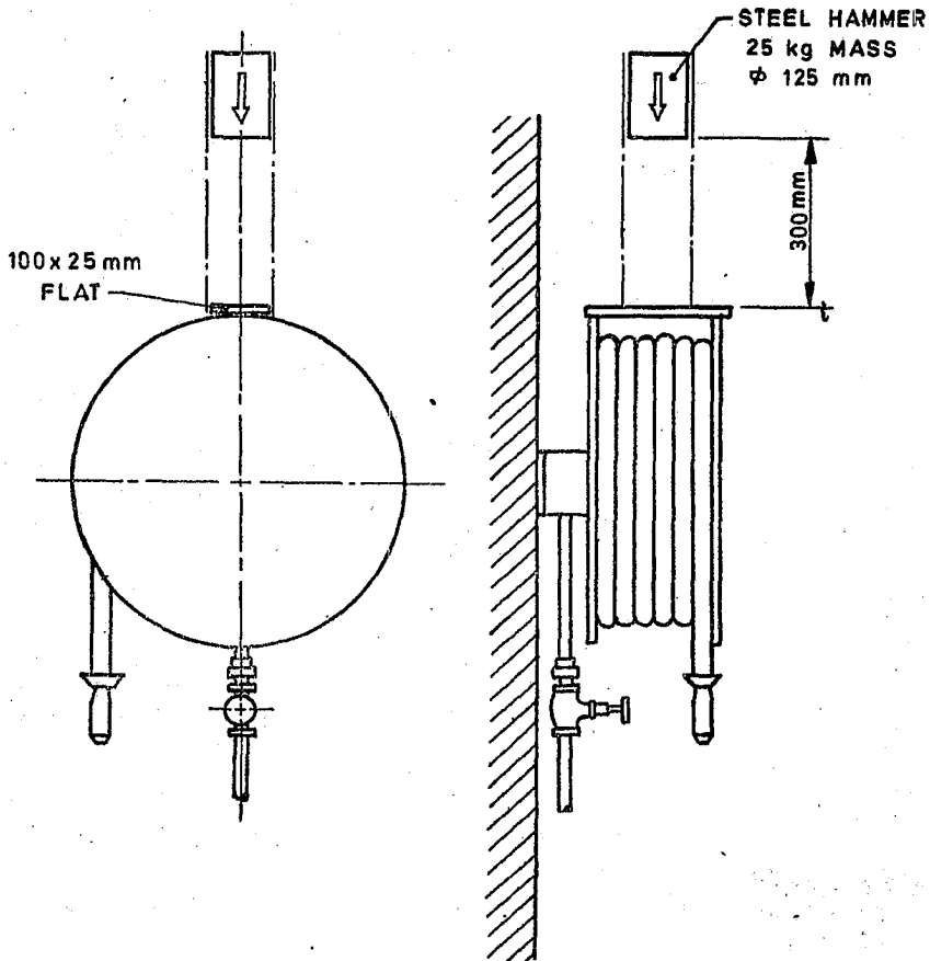
FIG. 3 DETAIL OF IMPACT TEST
