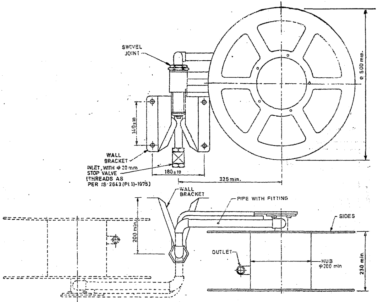
All dimensions in millimetres. FIG. 1 HOSE REEL SWINGING TYPE
