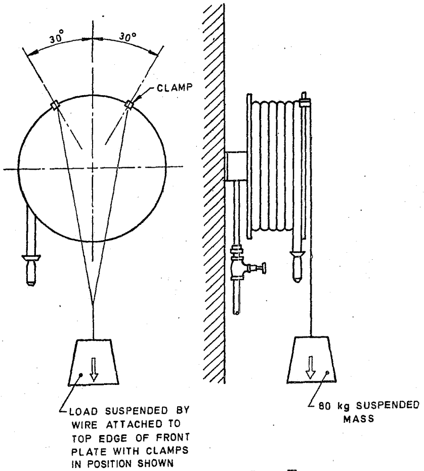
FIG. 4 DETAIL OF LOAD TEST
